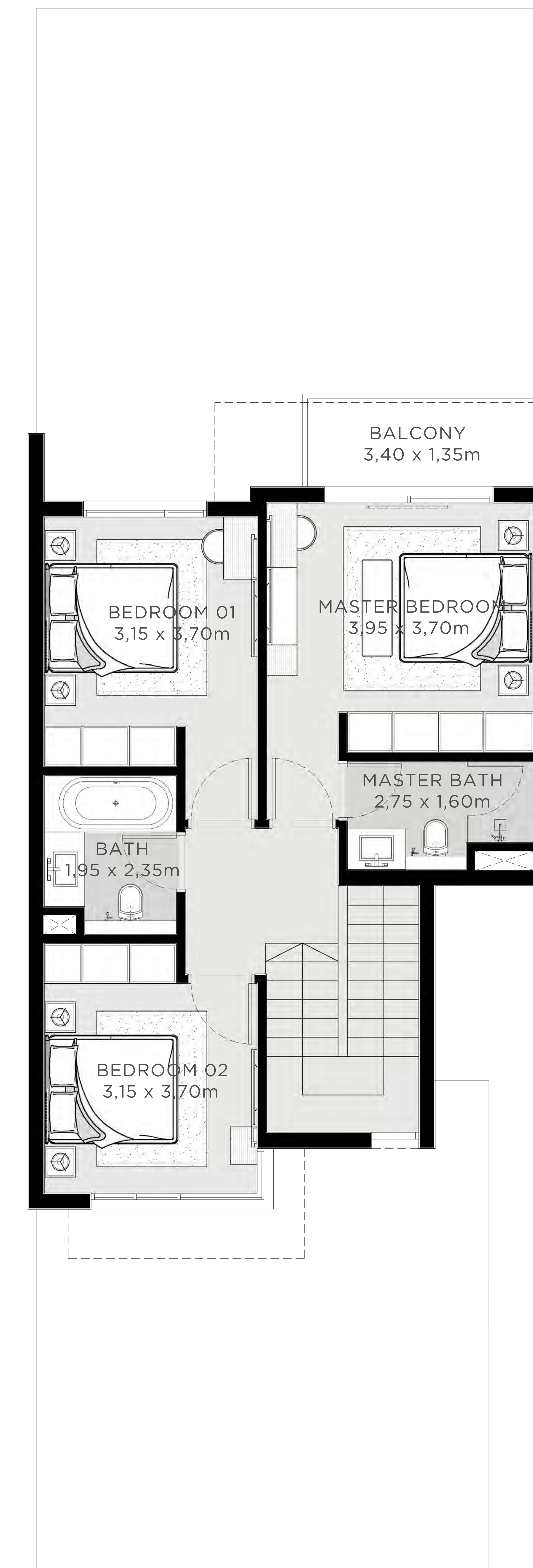
FIRST FLOOR
