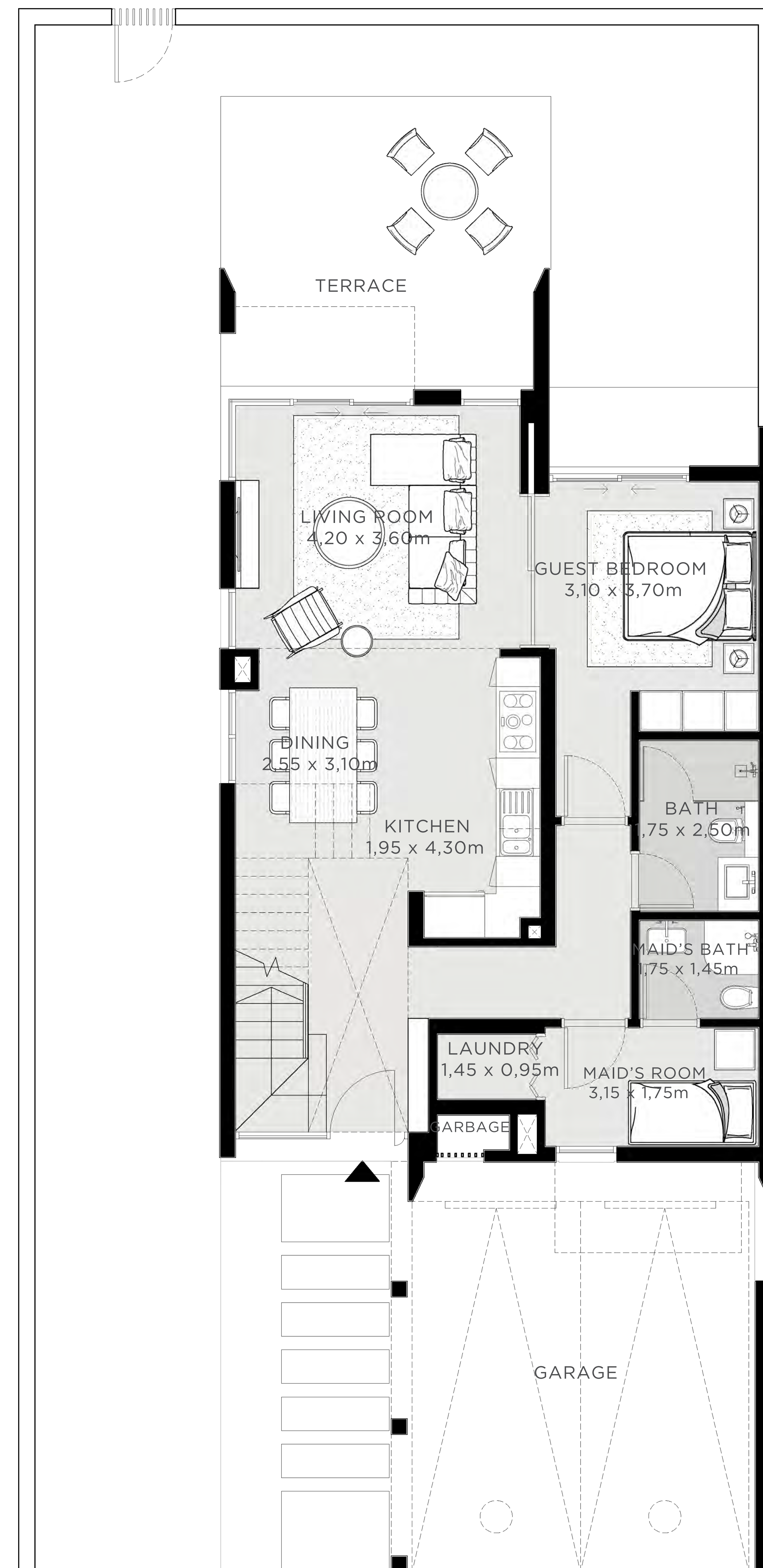
GROUND FLOOR
