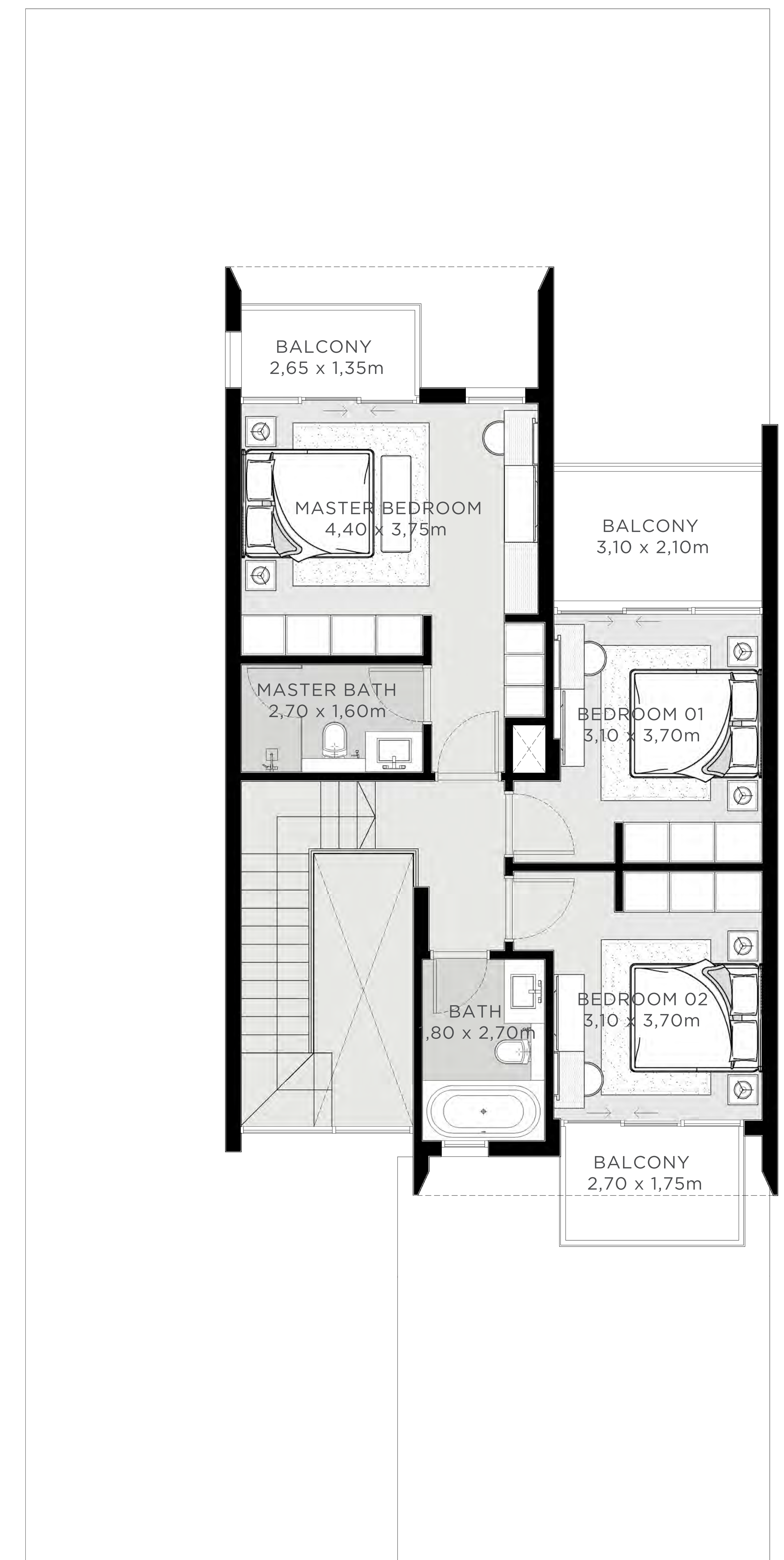
FIRST FLOOR
